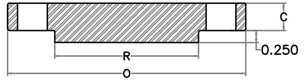
BLIND
