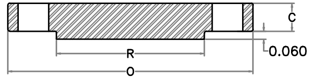
BLIND
