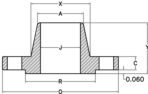
WELDING NECK
