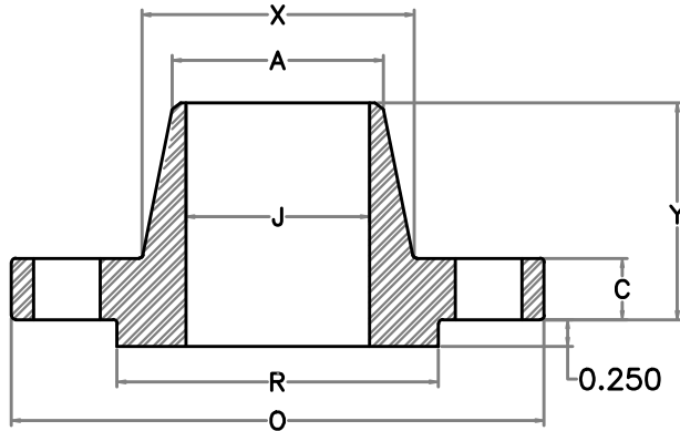
WELDING NECK
